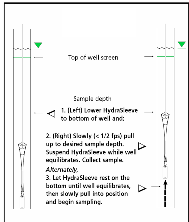
Figure 3-4. Bottom-up deployment.
