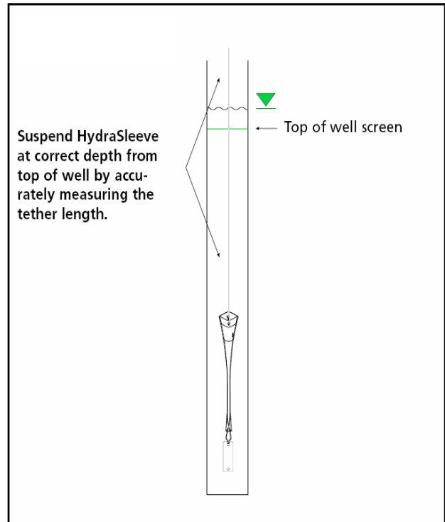
Figure 3-3. Top-down deployment.
